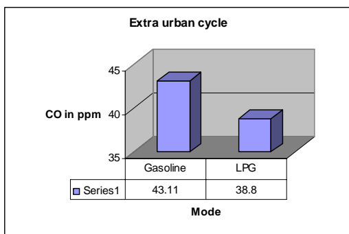
Fig. 5 Graph of CO in extra urban cycle
