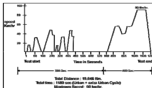
Fig. 3 Driving Cycle for emission measurement
