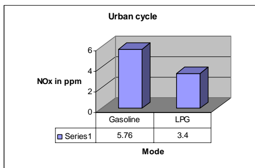
Fig. 8 Graph of NO x in urban cycle
