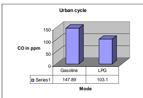
Fig. 4 Graph of CO in urban cycle
