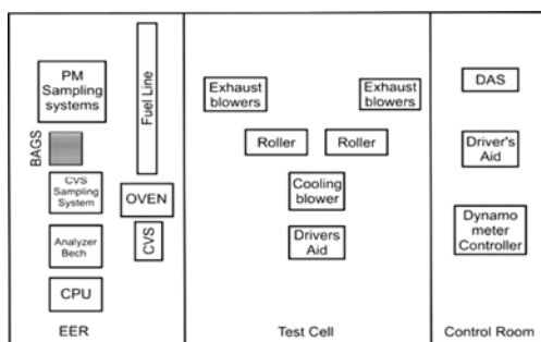
Fig. 2 Equipment layout for Emission testing
